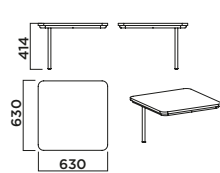
Corner table COD. 5095-TS2W L630 P630 H414
