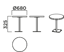
Side table COD. CA5095SO3 L680 P680 H325
