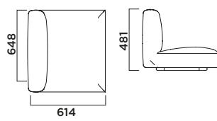
Cushion Module with backrest COD. CS02-5095 L648 P607 H481
