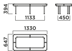
Two-seater structure module COD. CT5095SO2 L1330 P450 H394
