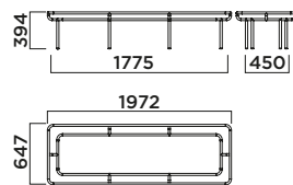
Three-seater structure module COD. CT5095SO3 L1972 P450 H394
