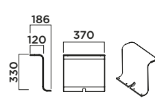
Upholstered Armrest COD. CA5095SO2 L370 P186 H330
