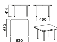
Free standing table COD. 5095-TS4W L630 P630 H414
