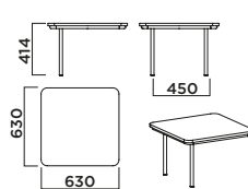
Side table COD. 5095-TS3W L630 P630 H414
